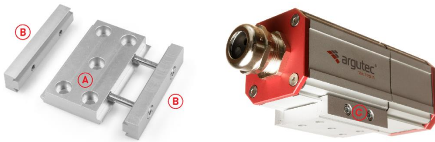
Figure 5 – Installing mounting kit
